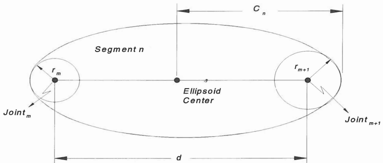
Figure 6 Ellipsoid Semiaxes
